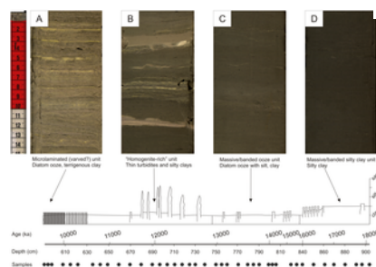
Figure 2. Core MAL05-2A lithostratigraphy within the study interval.
