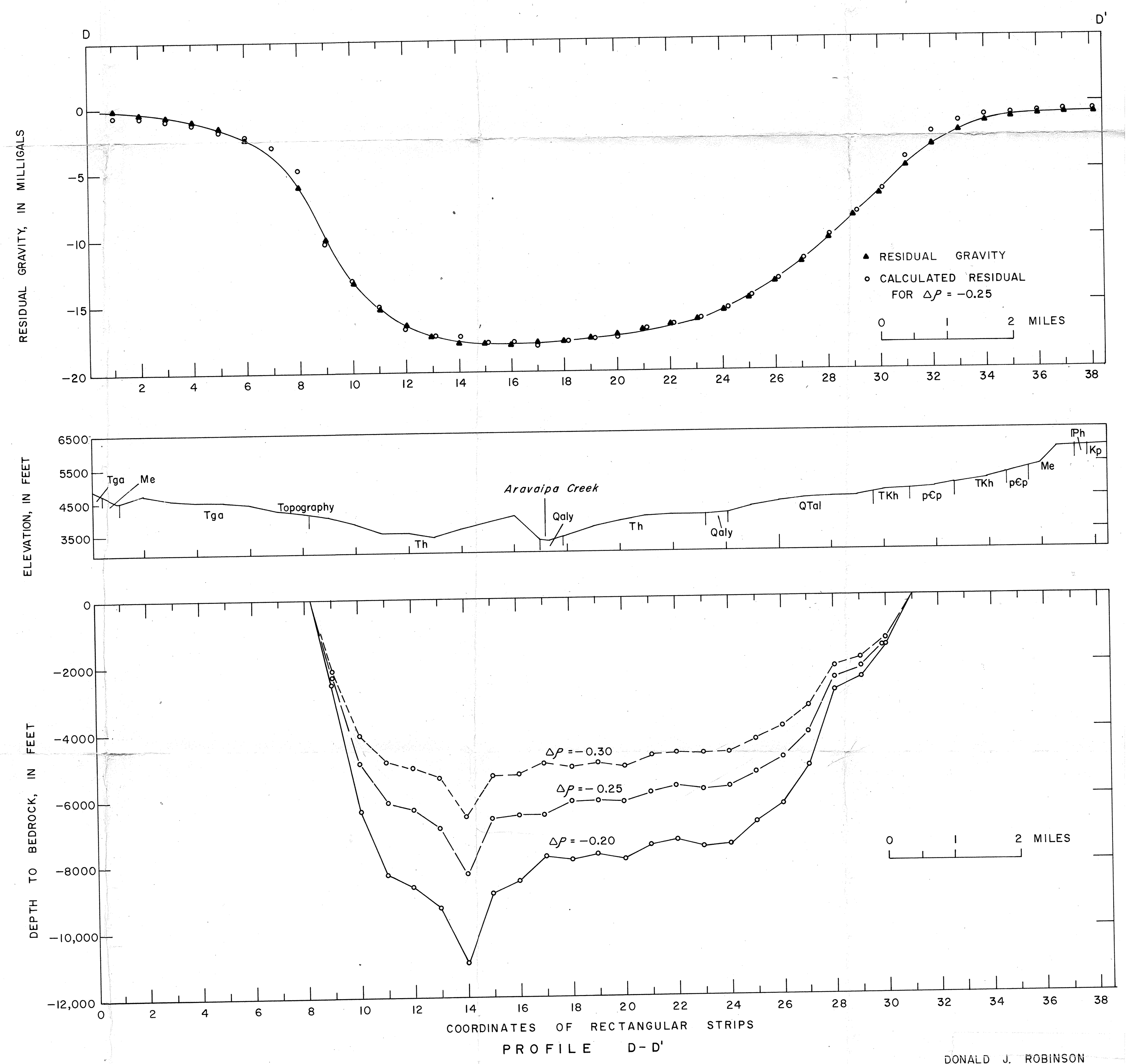
FIGURE II.--GRAVITY PROFILES FOR THE ARAVAIPA VALLEY AREA.
