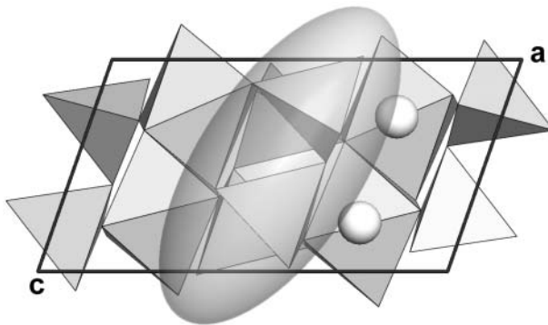
FIGURE 10. Oriented unit strain ellipsoid overlying a cartoon of the P2_1/c spodumene structure (3.342–8.835 GPa). Spheres represent Li atoms, and polyhedra are \text{SiO}_4 and \text{AlO}_6 .
