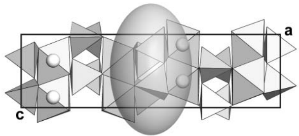
FIGURE 11. Oriented unit strain ellipsoid overlying a projection of Pbc_a enstatite down b . Spheres represent \text{Mg}(\text{M}2) atoms, polyhedra are \text{MgO}_6 and \text{SiO}_4 .
