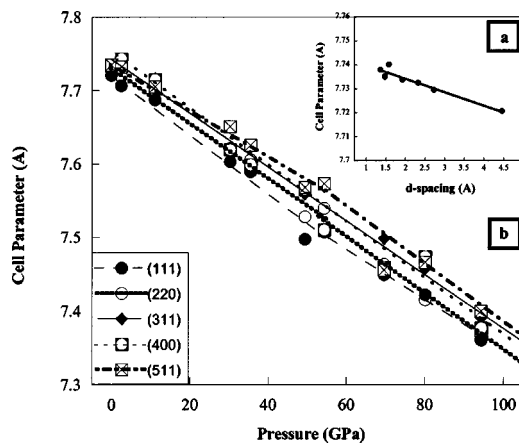
FIG. 1. (a) Relationship between d spacing and cell parameter ( a ) of nanocrystalline spinel \text{Si}_3\text{N}_4 at ambient conditions. (b) Pressure dependences of the cell parameter ( a ) calculated from the observed diffraction planes of nanocrystalline spinel \text{Si}_3\text{N}_4 . Note: Since the other peaks become broad and weak upon compression, a large error may exist, so we did not use those peaks in this plot.
