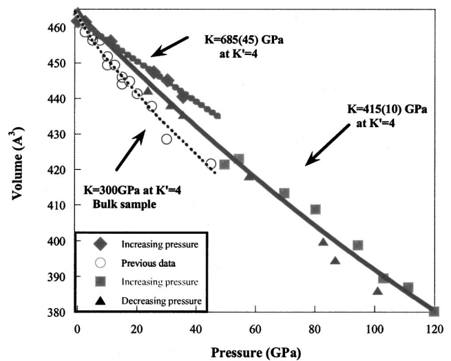
FIG. 2. The EOS curves fitted from the volumetric data obtained at pressures below and above 40 GPa, respectively. Note: Data obtained previously and at decompression in this study are also presented for comparison.
