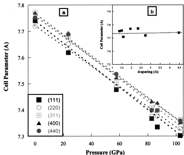
FIG. 3. (a) Pressure dependence of the cell parameter ( a ) calculated from the observed diffraction planes of nanocrystalline spinel \text{Si}_3\text{N}_4 upon release of pressure. Note: We did not use some broad low intensity peaks, as described in Fig. 1(b). (b) Correlation between d spacing and cell parameter ( a ) of the pressure-quenched nanocrystalline spinel \text{Si}_3\text{N}_4 .
